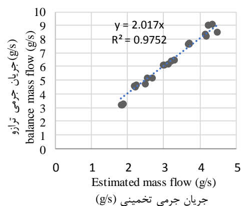
Figure (9) Results of mass flow estimation by monitoring system
