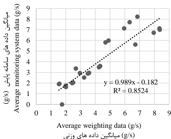
Figure (9) Results of mass flow estimation by monitoring system
