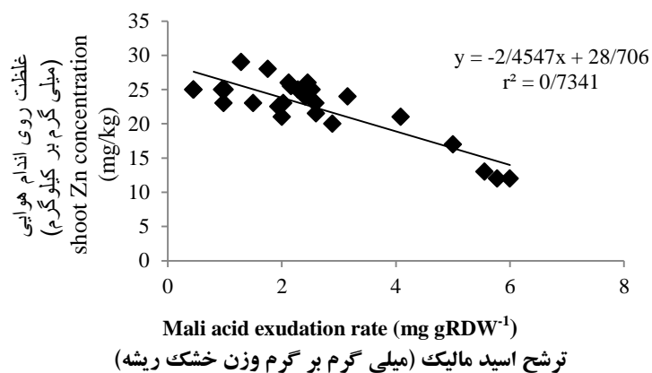
Figure (6) Correlation between shoot Zn concentration and MA exudation rate in 704 genotype
